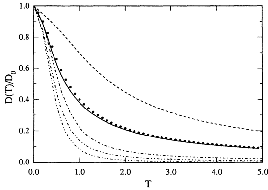
FIG. 3. D(T)/D_0 as a function of T for U/t = 2 . Numerical results are indicated by (\cdot \cdot \cdot -) L = 6 , (-\cdot \cdot \cdot -) L = 10 , (- \cdot \cdot \cdot -) L = 14 , and t_h = 0.5t ; points indicate t_h = t and L = 18 . The continuous line is the Bethe ansatz result and the dashed line D(T)/D_0 for a free particle.
