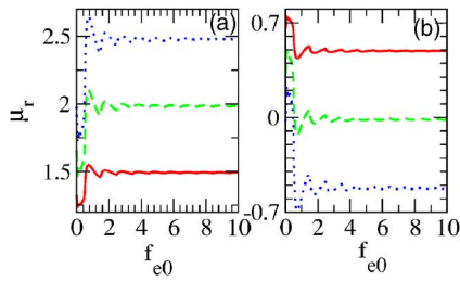
FIG. 4. (Color online) Relative permeability \mu_r vs f_{e0} , for \tilde{F}=0.01 (red-solid curves), \tilde{F}=0.02 (green-dashed curves), \tilde{F}=0.03 (blue-dotted curves), and (a) \Omega=0.99 ; (b) 1.01.
