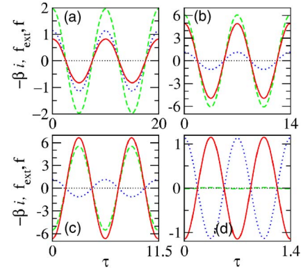
FIG. 3. (Color online) Time dependence of the flux f (green-dashed curves), the applied flux f_{\text{ext}} (blue-dotted curves), and the response \beta i (red-solid curves), for \beta=0.15 , \gamma=0.001 , f_{e0}=1.14 , and (a) \Omega=0.63 ; (b) \Omega=0.9 ; (c) \Omega=1.1 ; (d) \Omega=9.0 .
