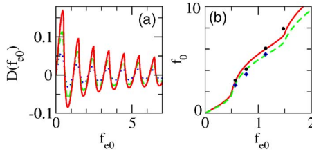
FIG. 2. (Color online) (a) Coefficient D vs the applied flux amplitude f_{e0} , for \beta=0.15 (red-solid curve); \beta=0.10 (green-dashed curve); \beta=0.05 (blue-dotted curve). (b) The amplitude of the flux f_0 vs f_{e0} , for \Omega=0.9 (red-solid curve), \Omega=1.1 (green-dashed curve), and \gamma=0.001 , \beta=0.15 . The black circles and blue diamonds correspond to the numerically obtained f_0 for \Omega=0.9 and 1.1 , respectively.
