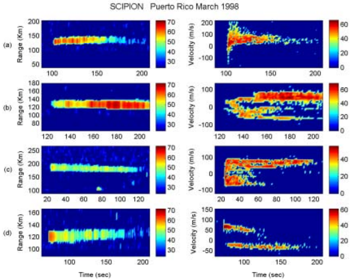
Figure 1. A meteor-induced backscatter echo (a) followed by three typical examples of meteor echoes characterized by a bifurcated Doppler spectrum, all observed with a 15 MHz radar. These echoes have long lifetimes ranging from many seconds to a few minutes
